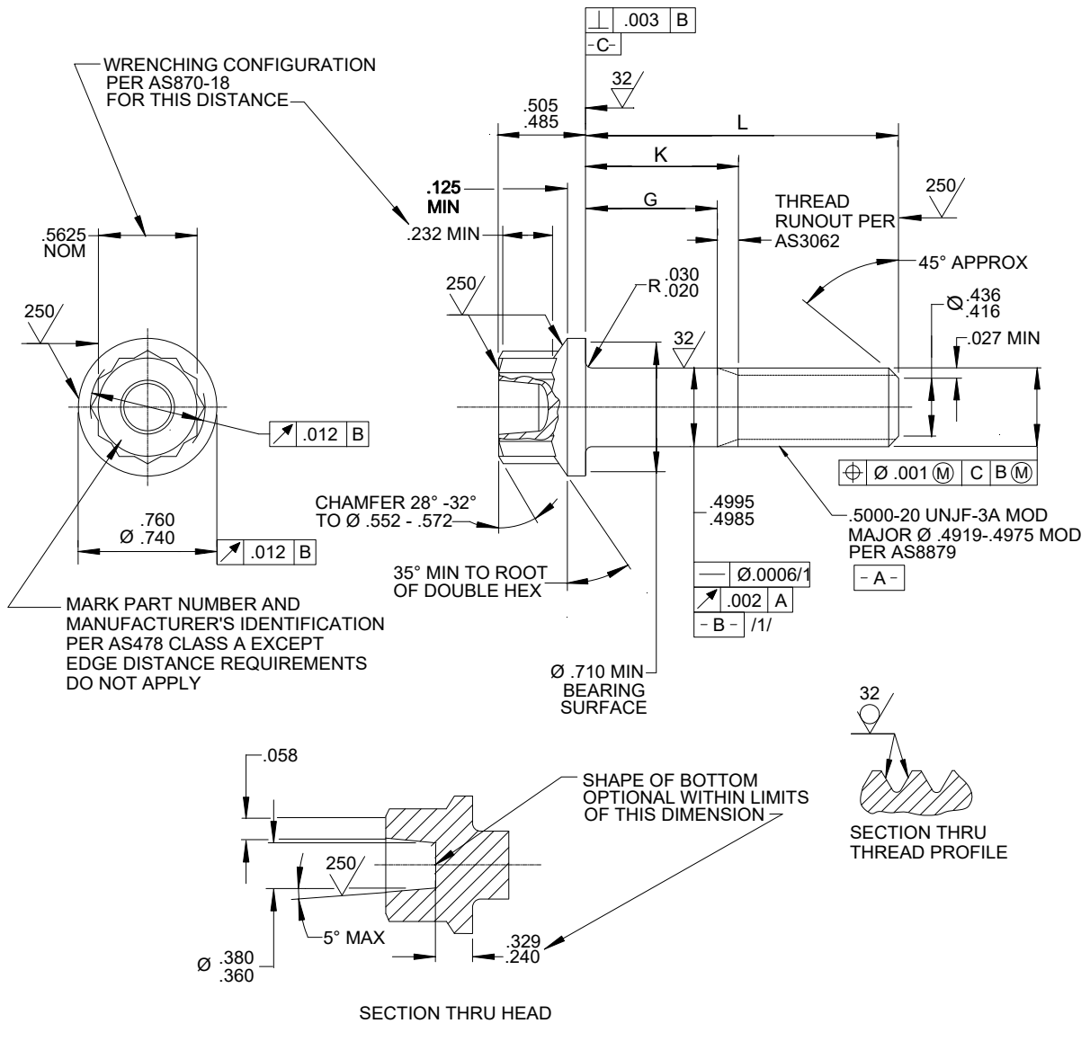
FIGURE 1 - BOLT
